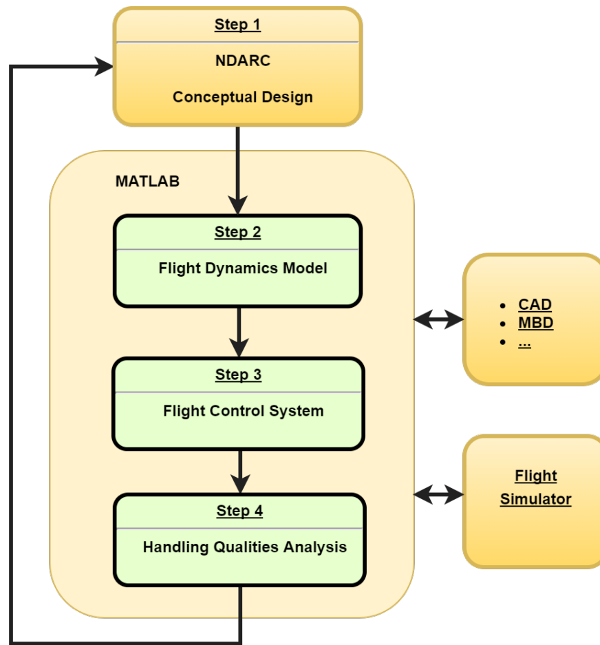
Fig. 1: Rotorcraft conceptual design tool architecture.
