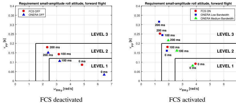
Fig. 13: Bandwidth and Phase Delay Comparison with [26].
