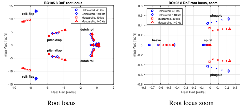
Fig. 5: Root locus comparison between BO105 8-DOF model and [18].
