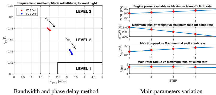
Fig. 15: Example of results with closure of the loop.
