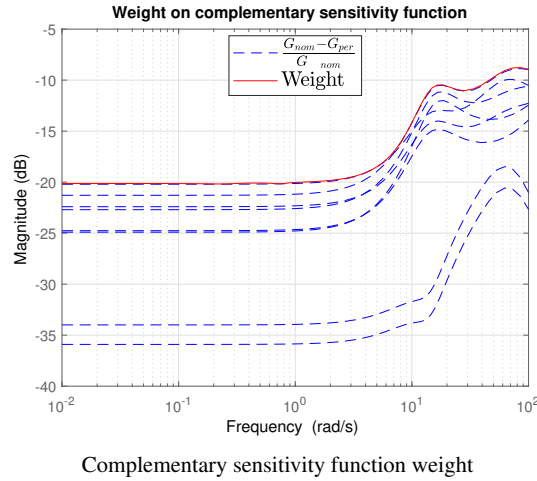
Fig. 11: Weights on sensitivity functions for regulator synthesis.
