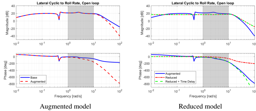
Fig. 7: Bode Plot for flight dynamics reduced models on roll axis.
