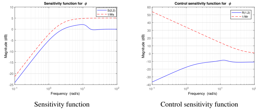
Fig. 9: Sensitivity and control sensitivity functions from regulator synthesis.
